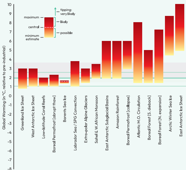
Earth system tipping points become possible, likely or very likely at varying levels of global warming. Credit: Armstrong McKay et al, "Exceeding 1.5°C global warming could trigger multiple climate tipping points", published in Science, 2022.
