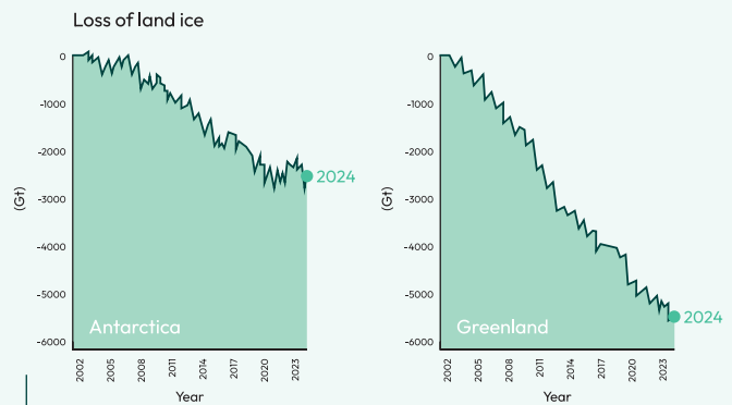
Graphs highlighting the loss of land ice in Antarctica and Greenland over a period of twelve years.
