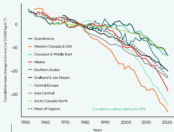
Figure 1. Melting of glaciers. Reducing mass of reference glaciers in regions worldwide. Sources: www.worldviewofglobalwarming.org ; World Glacier Monitoring Service
